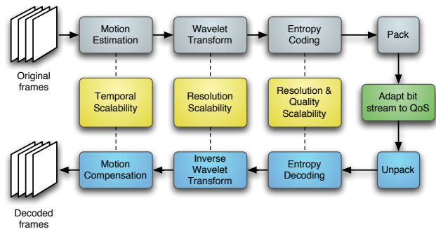
Figure 1. High-level overview of the codec.
